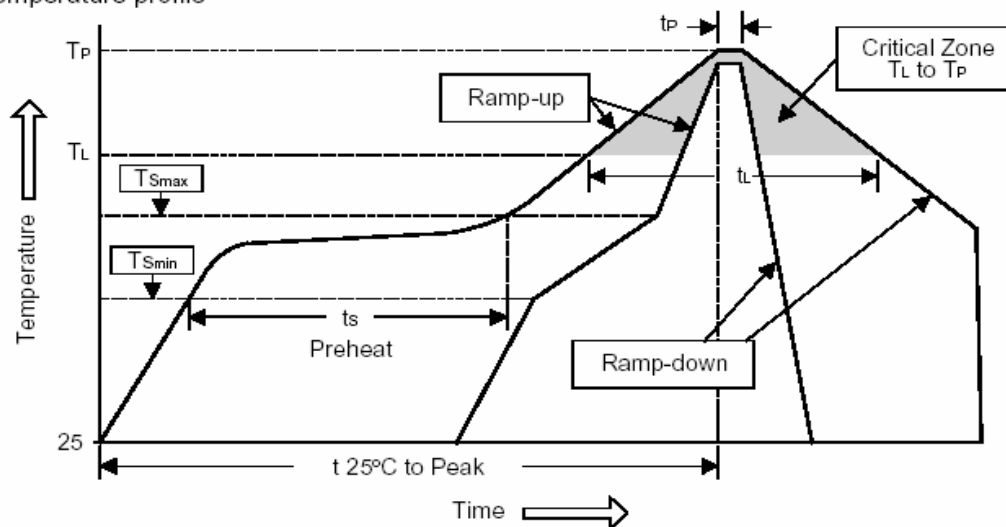
Figure 1: Temperature profile
